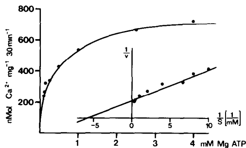
Fig.3. Dependence of calcium uptake velocity by isolated guinea pig parotid gland microsomes on the concentration of \text{ATP} \cdot \text{Mg}^{2+} . The calcium uptake was measured in the presence of oxalate.
